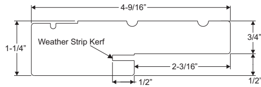
4-9/16" Pine, and Framesaver Jamb
