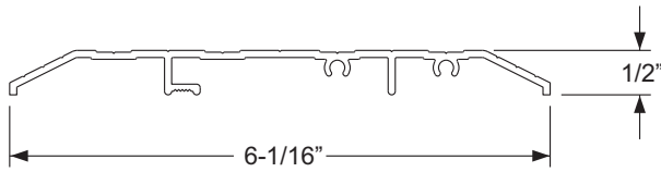
Aluminum Public Access Sill (Mill Finish)
