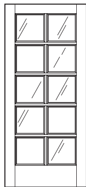
F7010 3/4" IG 1 3/8" TDL Bar 2'-0" x 6'-8" 3'-0" x 6'-8" 2'-6" x 6'-8" 2'-0" x 7'-0" 2'-8" x 6'-8"
