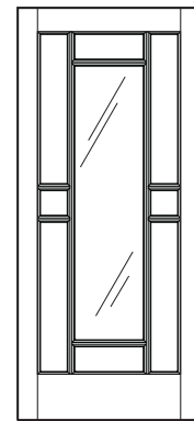
F7155 3/4" IG 1 3/8" TDL Bar 3'-0" x 6'-8" 2'-0" x 6'-8" 3'-0" x 7'-0" 2'-4" x 6'-8"
