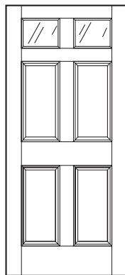
F2132 3/4" DHP Raised Panel Single pane safety 2'-8" x 6'-8" 3'-0" x 6'-8"
