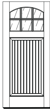
F7218 2'-6" x 6'-8" 2'-8" x 7'-0" 3'-0" x 6'-8" 3'-0" x 7'-0"
