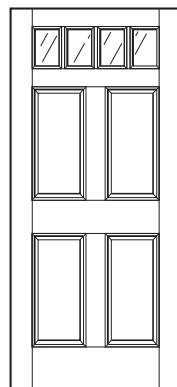
F2134 3/4" DHP Raised Panel Single pane safety 2'-6" x 6'-8" 3'-0" x 6'-8"
