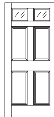
F4226 Clear IG 1-1/4" Raised Panel 3'-0" x 6'-8"
