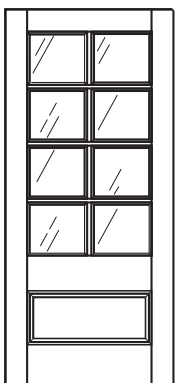
F7508 3/4" IG 1 7/16" Raised Panel 2'-0" x 6'-8" 2'-0" x 7'-0" 2'-6" x 6'-8" 2'-6" x 7'-0" 2'-8" x 6'-8" 2'-8" x 7'-0" 3'-8" x 6'-8"
