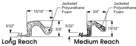
TT68LONGWSB (Bronze) TT68REGWSB (Bronze)
