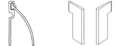
RAIN DEFLECTOR TTCORNERSEAL
