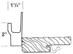
908 Brickmould PVC w/J
