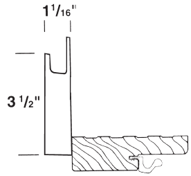
5/4 Flat PVC w/J
