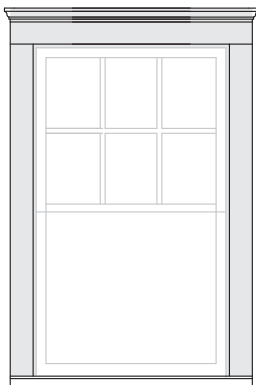
5/4 x 3 1/2 Flat Casing 5/4 x 5 1/2 Head Casing #7158 Rams Head Crown #7631 Sill Nosing
